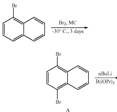
Reaction Scheme 1
