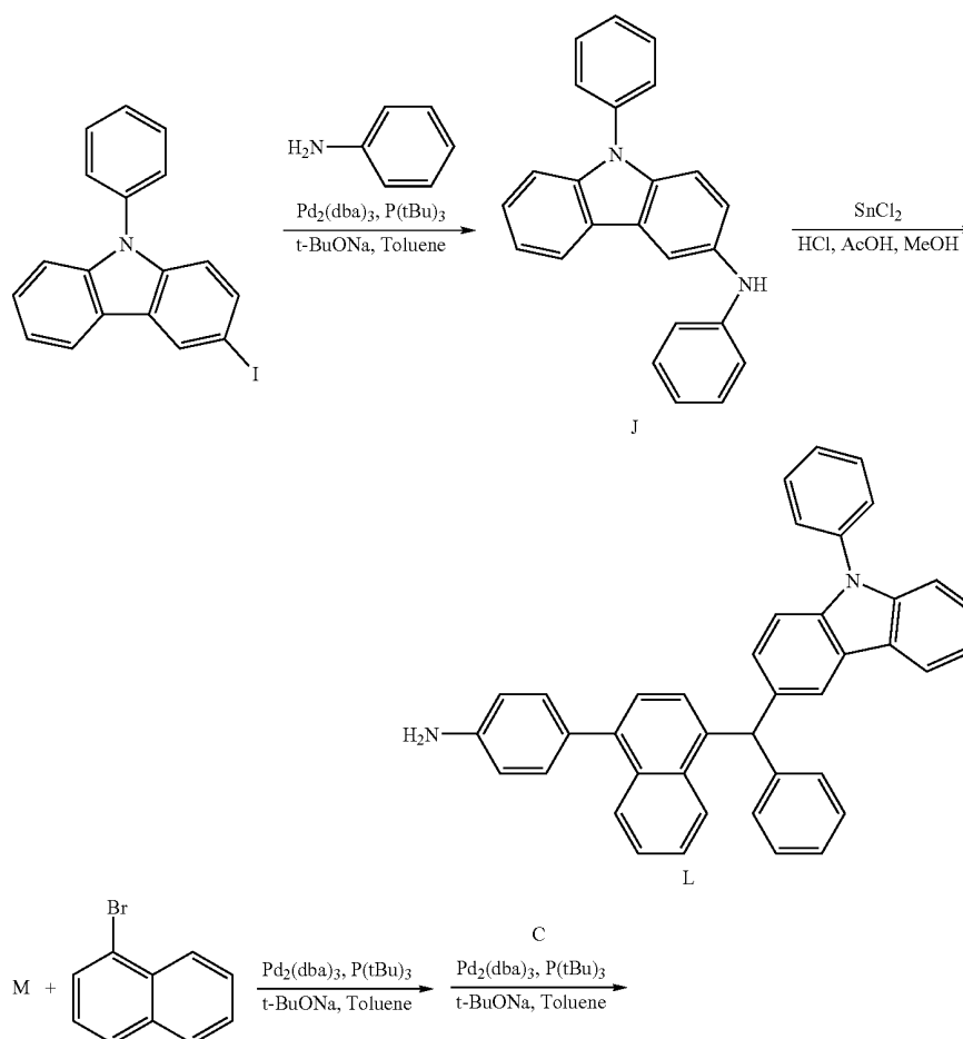
Reaction Scheme 3
