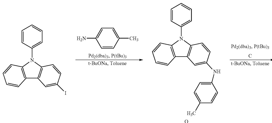
Reaction Scheme 5
