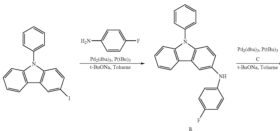
Reaction Scheme 6
